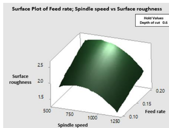
Figure (10): Effect of the interaction between Feed Rate and Spindle Speed on Surface Roughness.
